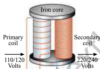
Fig: 16.18 (a) Step up transformer
