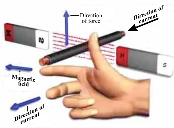
Fig: 16.5 Demonstration of the right-hand rule for conductors.
