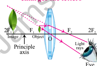
Fig: 13.18 (b) The ray diagram of a magnifying glass
