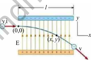
Fig: 17.14. Deflection of electron passing through uniform electric field
