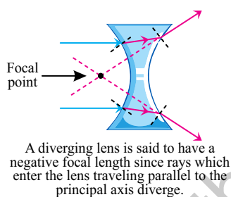
Refraction by a diverging lens
