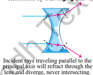
Refraction by a diverging lens
