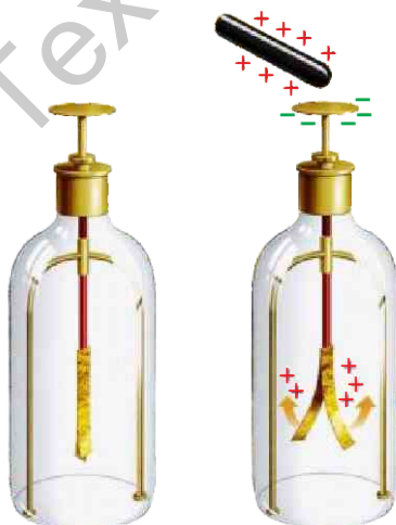
Fig: 14.7 Electroscope
